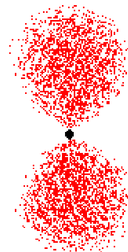
a p orbital
